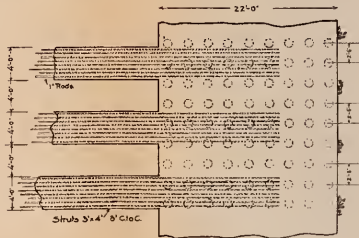
PLAN OF STRUTS & PILE FOUNDATION
